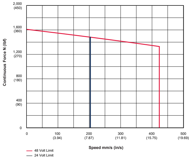
Exlar GTX060 - 02 5.08 mm (0.2 in) Screw Lead
