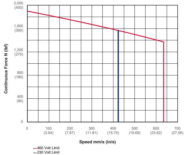
Exlar GTX060 0- 04 10.16 mm (0.4 in) Screw Lead
