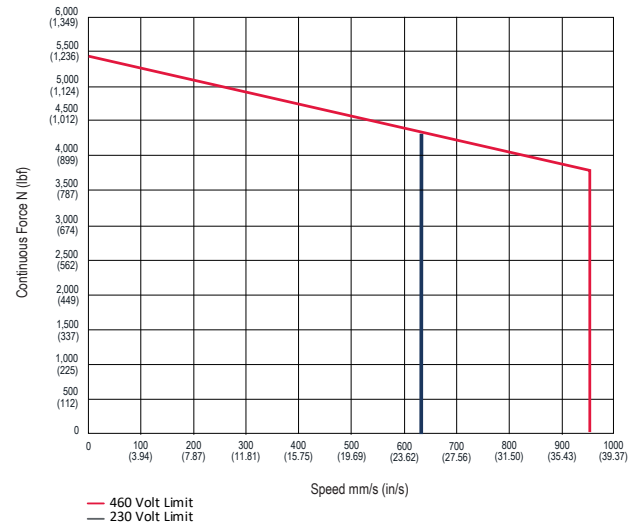
Exlar GTX100 - 05 12.7 mm (0.5 in) Screw Lead
