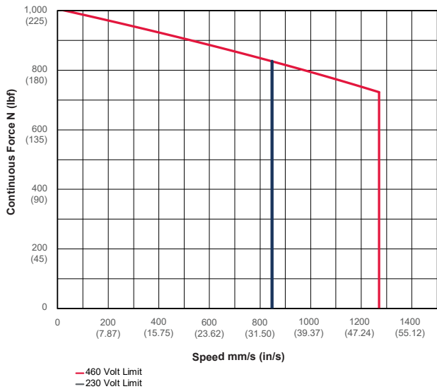
Exlar GTX060 - 02 5.08 mm (0.2 in) Screw Lead
