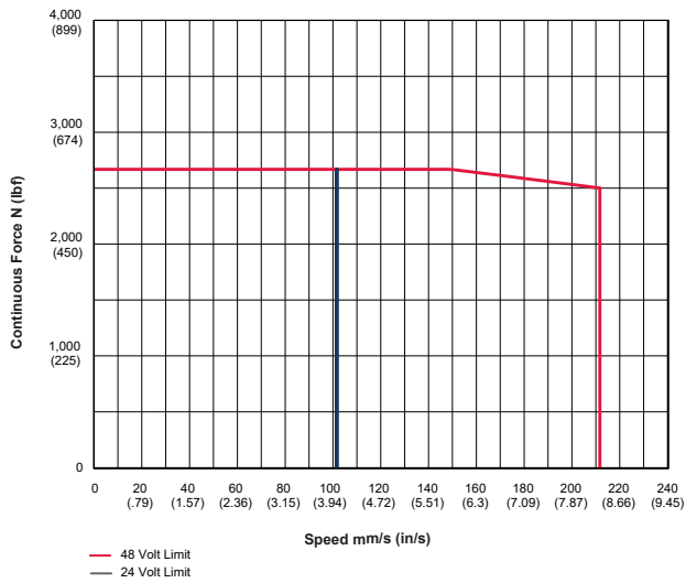
Exlar GTX060 - 01 2.54 mm (0.1 in) Screw Lead
