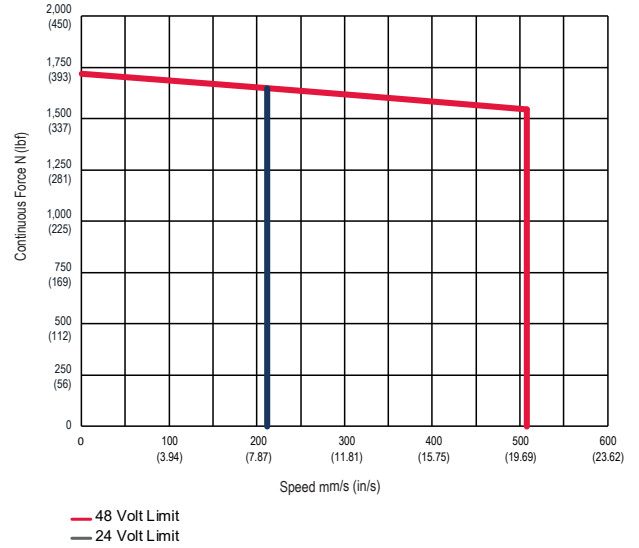
Exlar GTX080 0- 05 12.7 mm (0.5 in) Screw Lead
