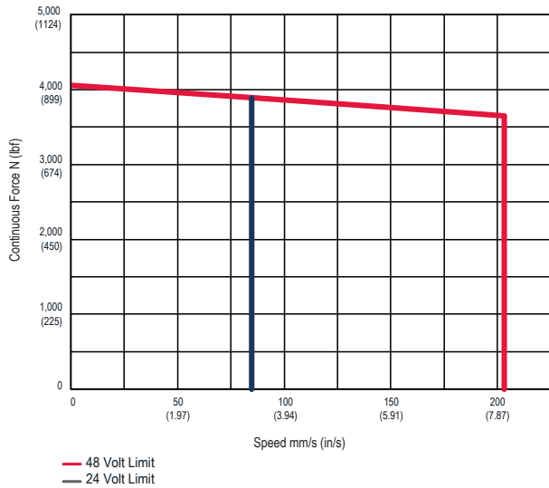
Exlar GTX080 - 02 5.08 mm (0.2 in) Screw Lead
