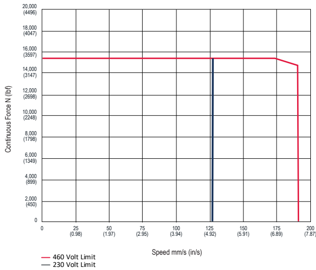
Exlar GTX100 - 01 2.54 mm (0.1 in) Screw Lead
