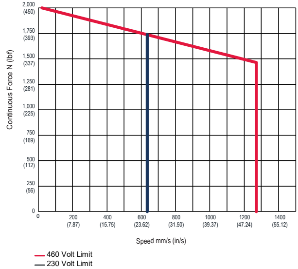
Exlar GTX080 - 05 12.7 mm (0.5 in) Screw Lead
