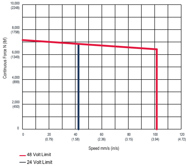
Exlar GTX080 - 01 2.54 mm (0.1 in) Screw Lead
