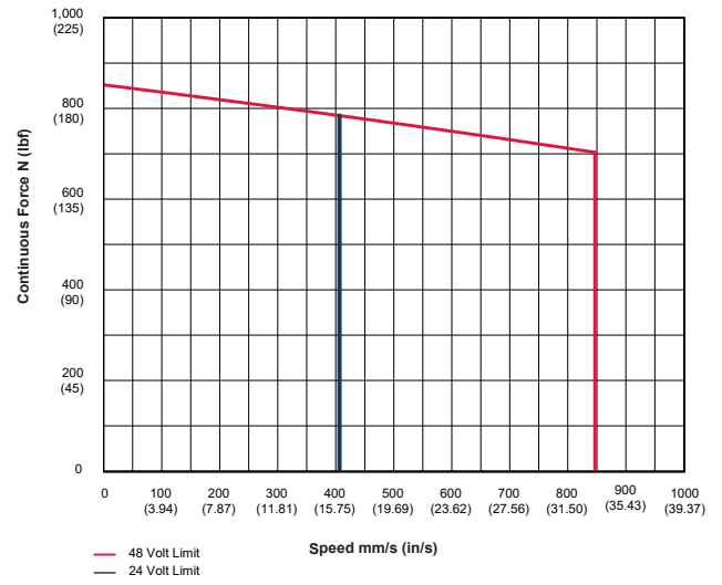
Exlar GTX060 - 04 10.16 mm (0.4 in) Screw Lead
