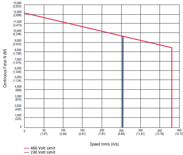
Exlar GTX100 - 02 5.08 mm (0.2 in) Screw Lead
