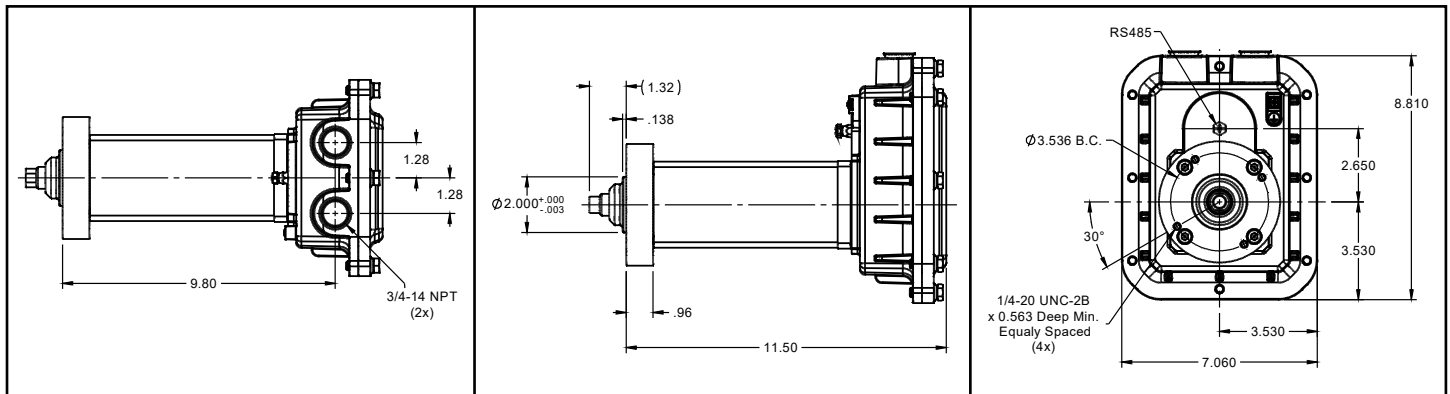
Tritex EVA080
